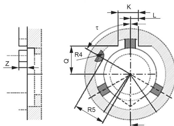
PY26d-1 ... PY26d7
