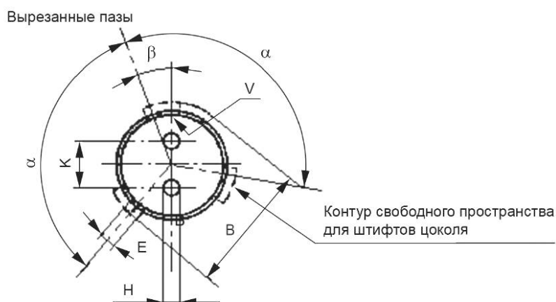
BA20s
