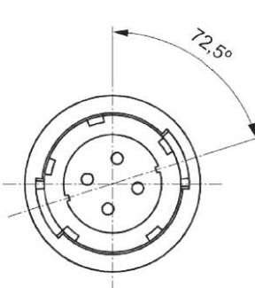
GR14q-3
