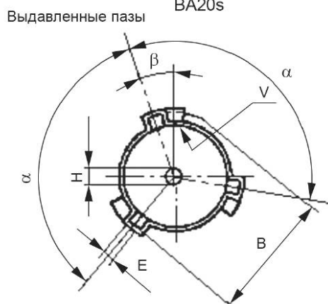
BA20s
