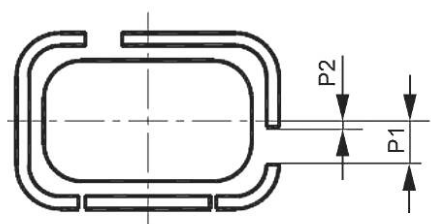
PG18.5d-4
