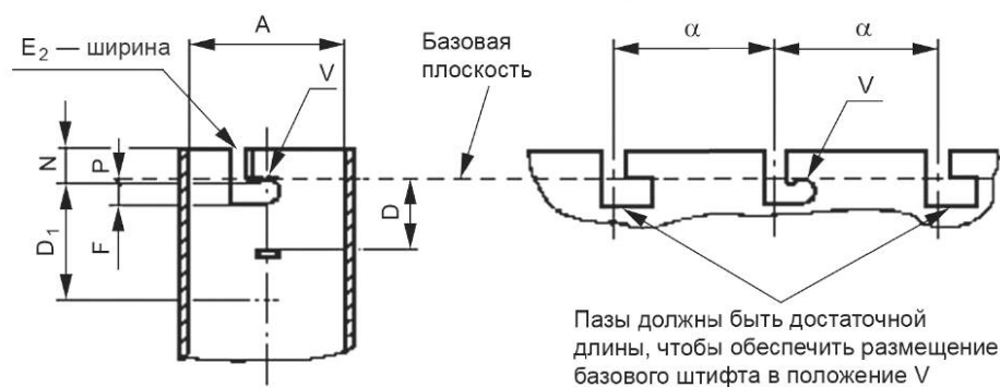
BA20d
