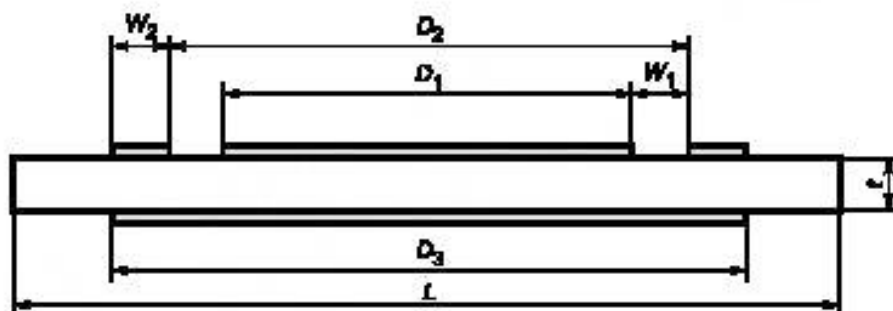
Рисунок 24 — Electrodes for measurements of volume and surface resistance
