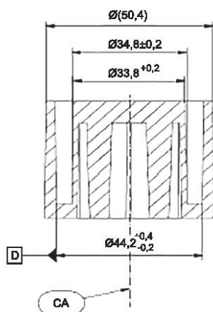
C-C (1:1)
