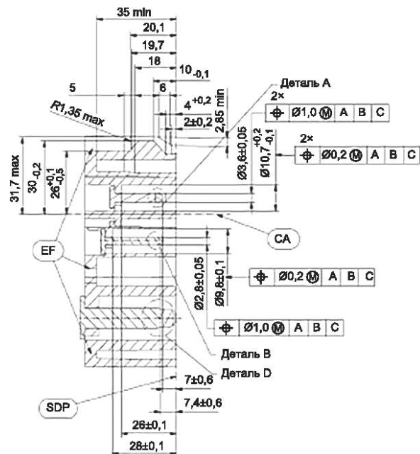
B-B (1:1)
